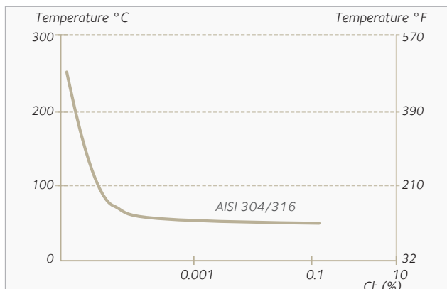
Constant strain tests in autoclave - Above the curve, SCC occurs
